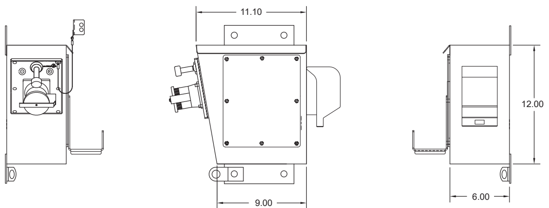
LEFT VIEW (SHOWN WITH CABLE MANAGEMENT BRACKET)
