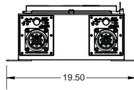
LEFT VIEW
