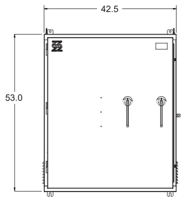
FRONT VIEW (HANDLE COVER NOT SHOWN)
